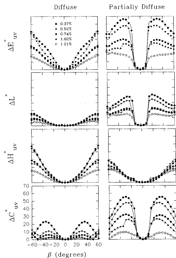
FIG. 4. Change in total color ( \Delta E_{uv}^* ), change in lightness ( \Delta L^* ), change in hue ( \Delta H_{uv}^* ), and change in chroma ( \Delta C_{uv}^* ) as a function of the viewing angle ( \beta ) for the polymer network stabilized cells using diffuse and partially diffuse illumination. All vertical and horizontal axes are scaled the same.
