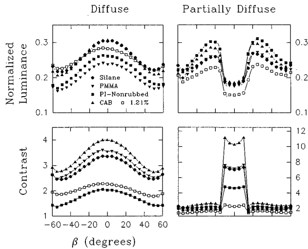
FIG. 5. Luminance and contrast as a function of the viewing angle ( \beta ) for the 1.21% polymer network stabilized cell and all surface stabilized cells using diffuse and partially diffuse illumination. All horizontal axes are scaled the same.
