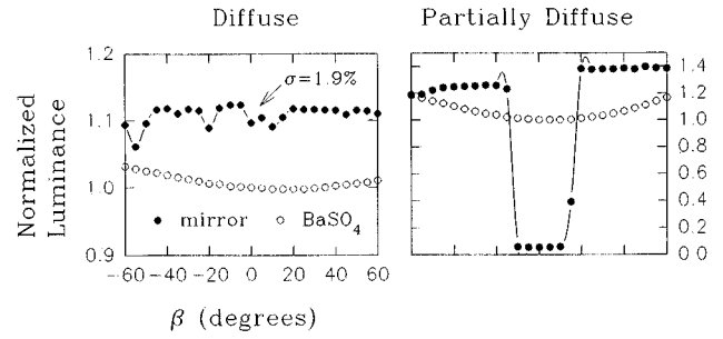
FIG. 2. Luminance as a function of the viewing angle ( \beta ) for a mirror and a white standard, BaSO 4 , using diffuse and partially diffuse illumination. The term \sigma denotes the standard deviation indicating the diffuse source is diffuse within \sim 1.9\% . The horizontal axes are scaled the same.
