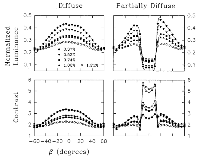
FIG. 3. Luminance and contrast as a function of the viewing angle ( \beta ) for the polymer network stabilized cells using diffuse and partially diffuse illumination. All horizontal axes are scaled the same.
