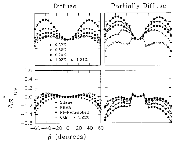
FIG. 7. Change in saturation ( \Delta S_{uv}^* ) as a function of the viewing angle ( \beta ) for all cells using diffuse and partially diffuse illumination. All vertical and horizontal axes are scaled the same.
