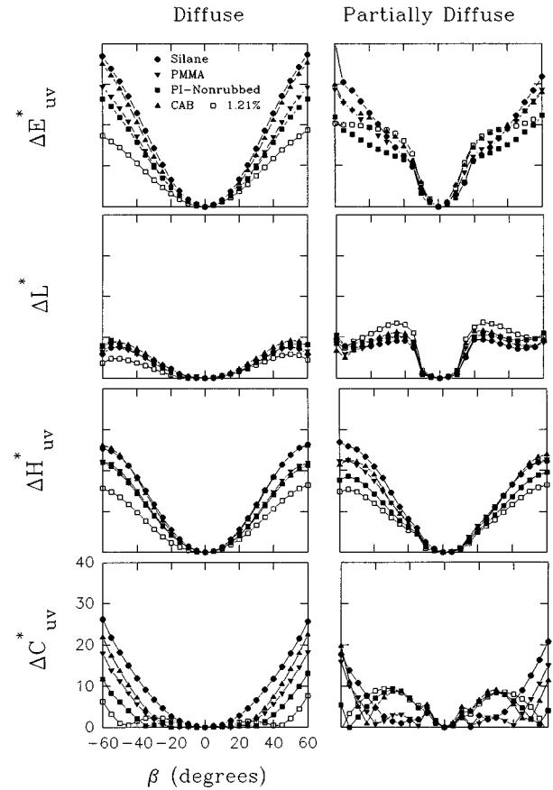
FIG. 6. Change in total color ( \Delta E_{uv}^* ), change in lightness ( \Delta L^* ), change in hue ( \Delta H_{uv}^* ), and change in chroma ( \Delta C_{uv}^* ) as a function of the viewing angle ( \beta ) for the 1.21% polymer network stabilized cell and all surface stabilized cells using diffuse and partially diffuse illumination. All vertical and horizontal axes are scaled the same.
