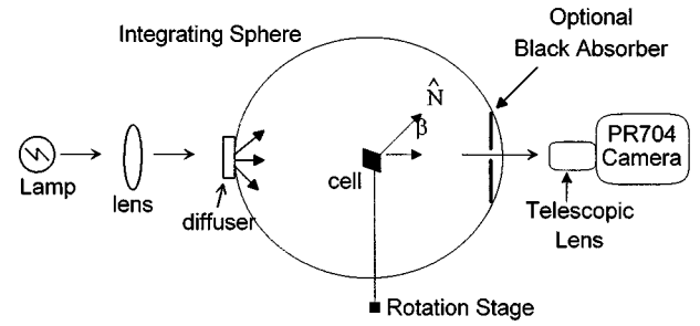
FIG. 1. Experimental apparatus for diffuse and partially diffuse lighting. Partially diffuse illumination is accomplished by placing the optional black absorber, with a small aperture in the center, internal to the integrating sphere in front of the exit aperture.
