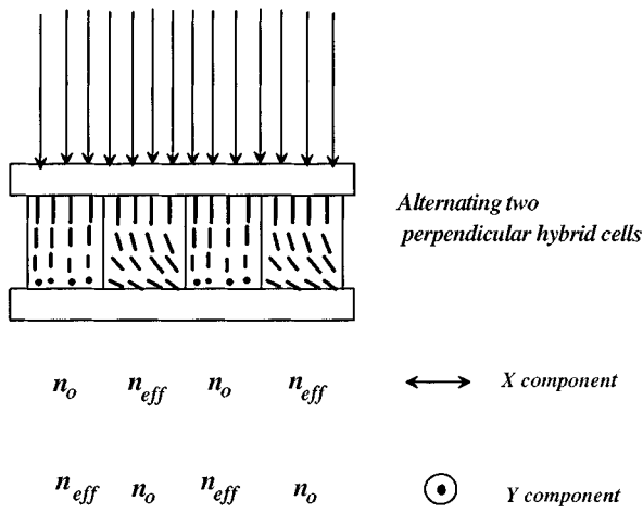
FIG. 2. New liquid crystal diffraction structure.
