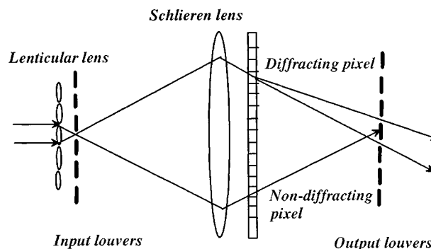
FIG. 1. Principle of a Schlieren optical projection system.
