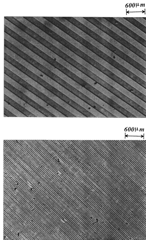
FIG. 4. Micrographs of two test cells with stripe widths of 200 and 24 μm, respectively.
