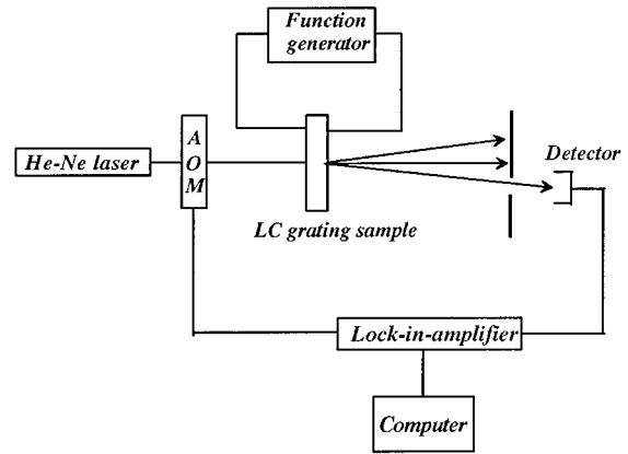
FIG. 3. Schematic of setup used to measure the electro-optical properties of test cells. (AOM) acoustic optical modulator.
