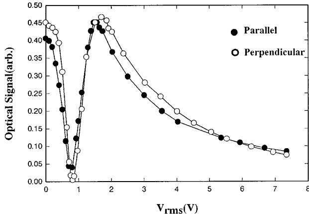
FIG. 6. Electro-optical data of first-order diffraction for the same test cell as Fig. 5 under two input polarization directions, one parallel to stripes and one perpendicular.
