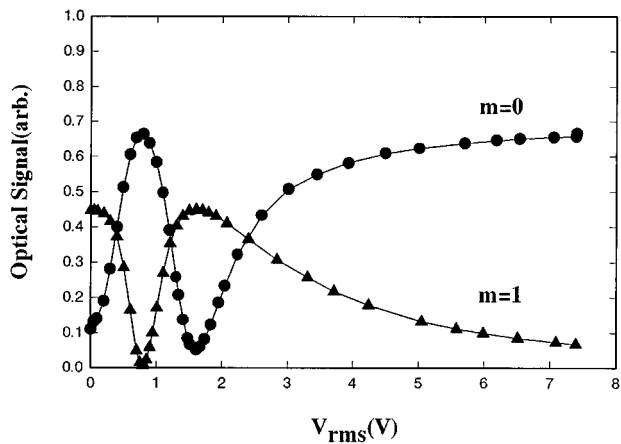
FIG. 5. Electro-optical data for zero and first diffraction order. The test cell stripe width is 75 \mu\text{m} and unpolarized laser light is used.
