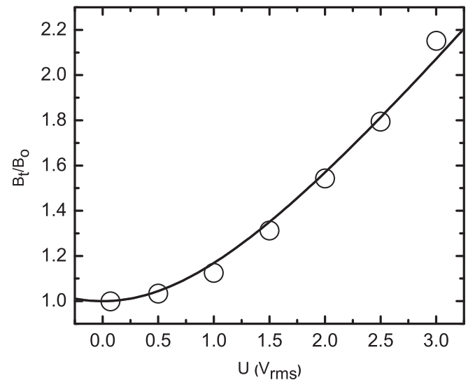
FIG. 6. Threshold magnetic field for splay-bend Freedericksz transition in CIPbis10BB determined as a function of voltage applied across the sample cell ( T_{IN} - T = 2^\circ\text{C} ). The E and B fields are parallel to each other and normal to the undistorted director. The solid line is a fit to Eq. (11) in the text.
