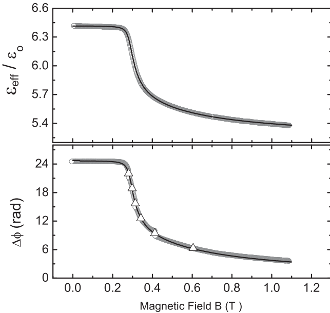
FIG. 5. Top panel: Effective dielectric constant of CIPbis10BB measured as a function of applied magnetic field B in the “splay” Freedericksz geometry and for T_{IN} - T = 2^\circ\text{C} . The vertical axis intercept corresponds to the value of \epsilon_{\perp}/\epsilon_0 . The solid line is a fit to Eq. (10) of the text. Bottom: Data for the phase shift \Delta\phi between ordinary and extraordinary components of polarized light transmitted through the sample as a function of applied B . The solid line is a fit to Eq. (8). The triangular symbols correspond to values of \Delta\phi where the intensity in Eq. (7) is a maximum.
