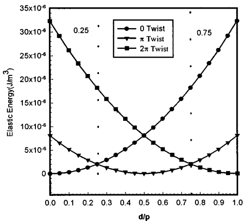
FIG. 2. Energy distribution for liquid crystal ZLI-4792 at 0^\circ pre-tilt angle.
