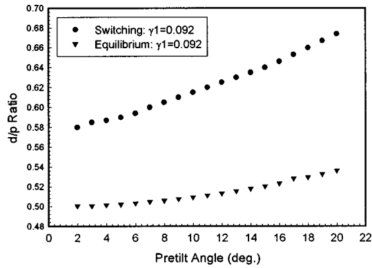
FIG. 5. The difference between switching and equilibrium d/p ratio with respect to pre-tilt angle.
