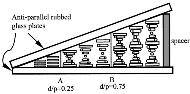
FIG. 1. Side view of liquid crystal twist states in a wedge cell.
