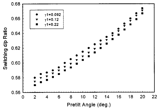
FIG. 6. The switching d/p ratio with different liquid crystal viscosities.
