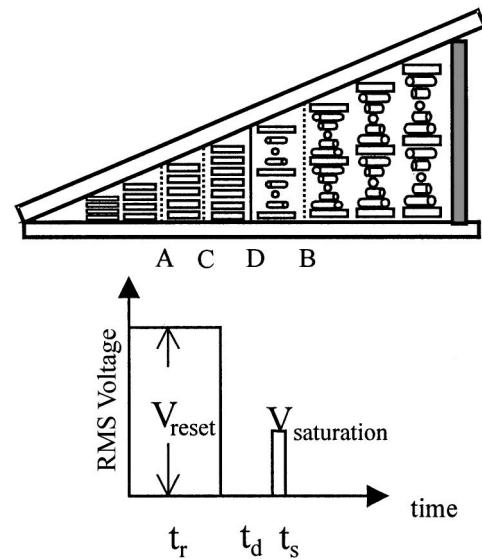
FIG. 3. Addressing waveform applied to the wedge cell.
