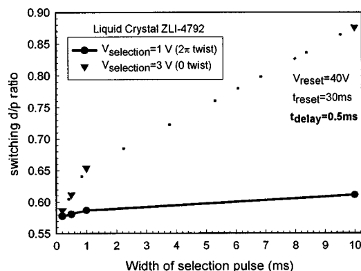
FIG. 8. The d/p switching window width of selection pulse.
