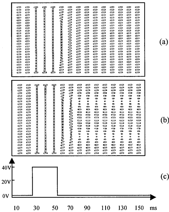
FIG. 4. Switching d/p ratio obtained by Berreman modeling software (a) d/p=0.585 , \theta_{\text{pret}}=5^\circ , (b) d/p=0.589 , \theta_{\text{pret}}=5^\circ , (c) addressing waveform with only reset pulse.
