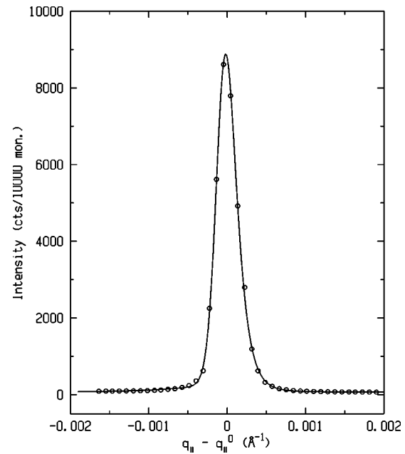
FIG. 2. Arm-zero profile. The solid line is the best fit to a sum of three Lorentzians. Full width at half-maximum is 2.6 \times 10^{-4} \text{ \AA}^{-1} .
