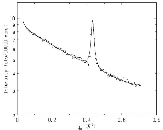
FIG. 3. Longitudinal scan of the empty beryllium cell yields the angular dependence of the background consisting of a well-defined peak due to the beryllium cell and upstream windows. The solid line is the best fit to Eq. (1). The beryllium peak is positioned at 0.433 \text{ \AA}^{-1} and has \text{FWHM} = 8.7 \times 10^{-3} \text{ \AA}^{-1} .
