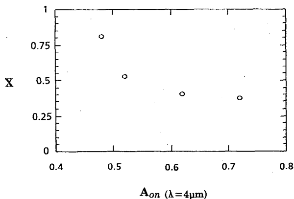
FIG. 5. The calculated fraction of liquid crystal in droplets in a PDLC composed of E7 and PVP as a function of the ON state scattering intensity measured at 4 \mu\text{m} .
