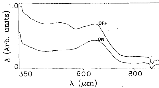
FIG. 2. The absorption spectra of an 18- \mu\text{m} -thick black PDLC shutter containing a black dichroic dye mixture of Y2, R4, R5, and B3 in the ON and OFF states.
