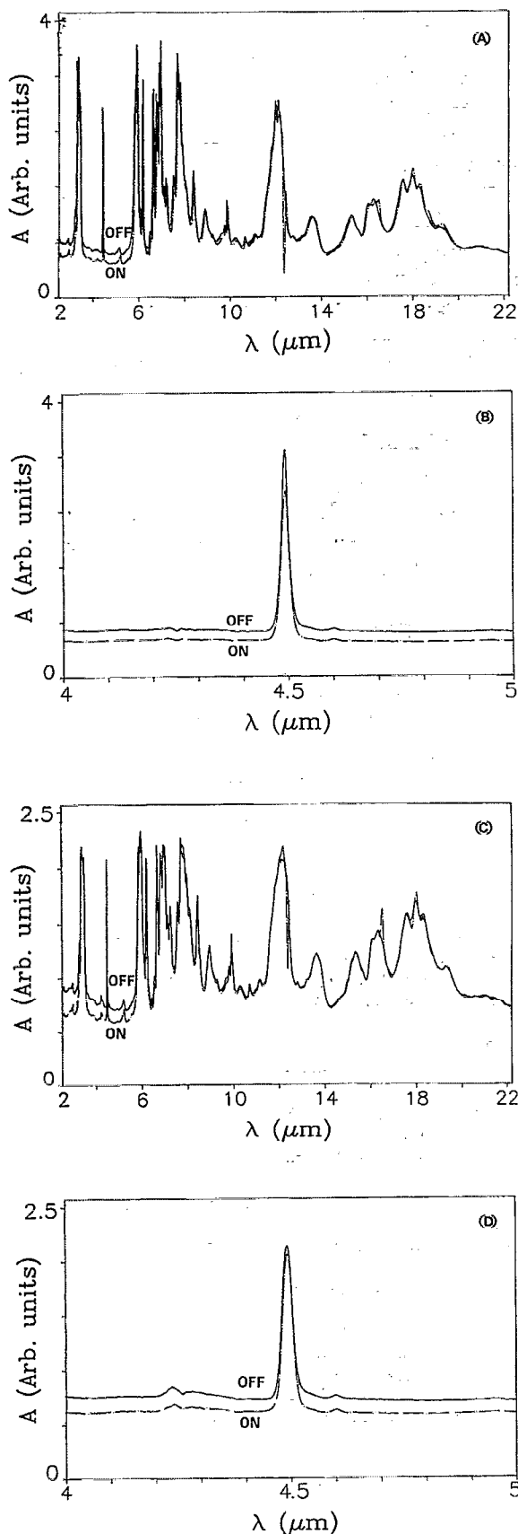
FIG. 4. ON and OFF state IR absorption spectra of a PDLC shutter formed from E7 and PVP cooled at 1 °C min for the 2–22 μm wavelength region (A) and for the 4–5 μm wavelength region, (B), and for the same shutter cooled at 2 °C min for the 2–22 μm wavelength region (C) and for the 4–5 μm wavelength region (D).
