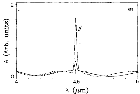
FIG. 3. IR absorption spectra for the eutectic liquid crystal mixture E7 for light polarized parallel, \parallel , and perpendicular, \perp , to the liquid crystal director; for the 2–22 \mu\text{m} wavelength region (A) and for the 4–5 \mu\text{m} wavelength region (B).
