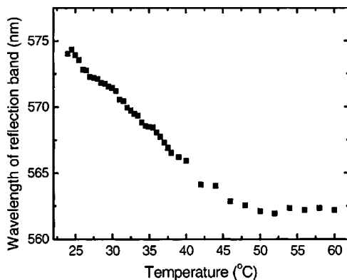
FIG. 2. Wavelength of the reflection band edge vs temperature for the undoped CLC (sample 1).
