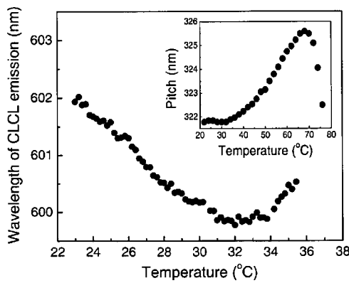
FIG. 1. Wavelength of CLC laser emission coupled to fiber vs temperature for sample 1. The inset presents pitch vs temperature.
