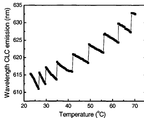
FIG. 3. Wavelength of CLC laser emission (sample 2) vs temperature.
