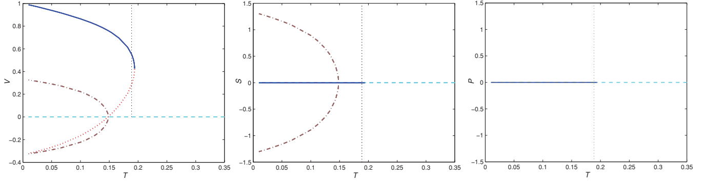
FIG. 1. (Color online) Solutions of the self-consistent equations in 4D for the scalar order parameters. Temperature is in units of k/\rho U .
