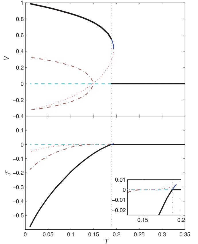
FIG. 2. (Color online) Free energy density of the three sets of solutions vs temperature in 4D.
