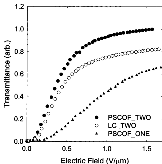
FIG. 5. Transmission vs applied field for the one substrate (PSCOF-ONE), two-substrate (PSCOF-TWO), and normal IPS cell (LC-TWO).
