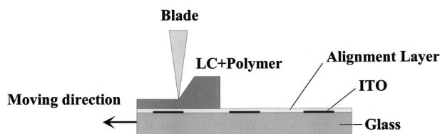
FIG. 1. Schematic illustration of the fabrication process.
