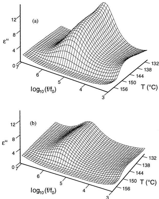
FIG. 2. Dielectric losses as the function of temperature and frequency ( f_0=1 Hz) for a 10\ \mu\text{m} cell. (a) Homochiral state, (b) racemic state. In the low frequency part the slight increase is due to freely moving ions. The increase at about 10 MHz is connected to the ITO layer.
