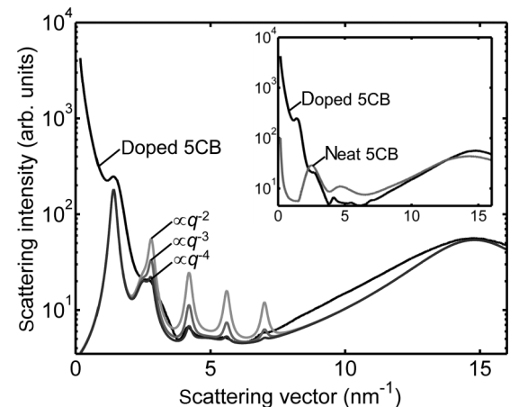
FIG. 2. Experimentally recorded scattering curve of nanoparticle-doped 5CB and three model curves with Bragg peak amplitudes proportional to q^{-2} , q^{-3} , and q^{-4} , respectively. The inset shows the scattering curves of the nanoparticle-doped and neat 5CB in comparison. The shown scattering curves were recorded at a temperature of 28 °C. The data were acquired with x-ray photon energy of 8 and 12 keV and a sample or detector distance of 120 (SAXS region) and 26 cm (WAXS region), respectively. The two sets of data were then merged by matching at q = 1.5 nm ^{-1} .
