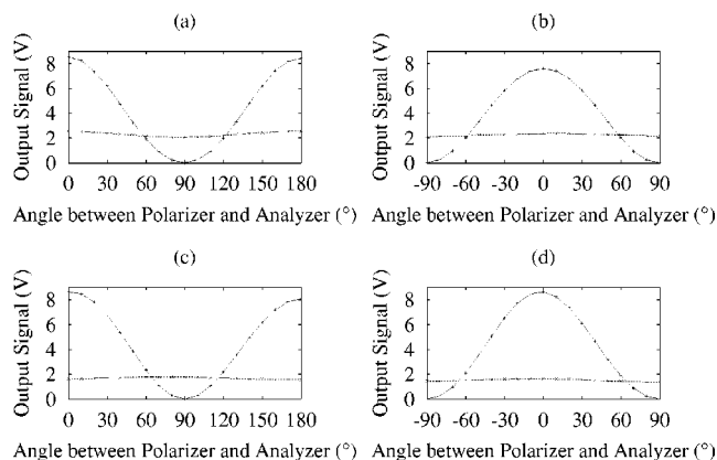
FIG. 1. The transmitted voltage vs angle between the polarizer and analyzer for no depolarizers and two types of depolarizers and incident polarization vertical [(a) and (c)] and horizontal [(b) and (d)]. In all four panels the larger voltage corresponds to no depolarizer present. Panels (a) and (b): K15 and 2.6% Antimony depolarizer (47 μm spacing). Panels (c) and (d): E7 and 2.4% large silica colloid depolarizer (16 μm spacing).
