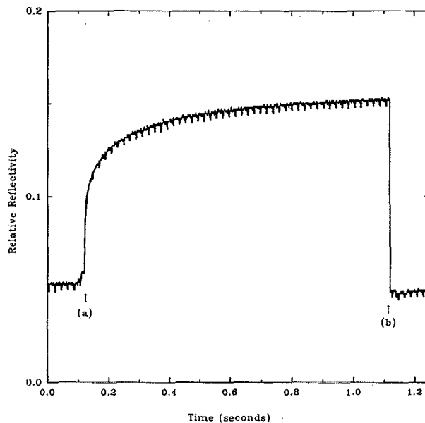
FIG. 3. The optical reflectivity of a CPD shutter plotted as a function of time. A 130 volt dc pulse of 20 ms duration is applied at point (a). An 80 V dc pulse of 20 ms duration is applied at point (b).
