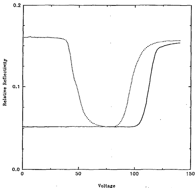
FIG. 4. Optical reflectivity of a CPD shutter initially in either the planar (dotted line) or focal conic (solid line) state plotted as a function of the voltage of an applied pulse. The voltage pulse is 20 ms in duration. The optical reflectivity is measured 800 ms after application of the pulse.
