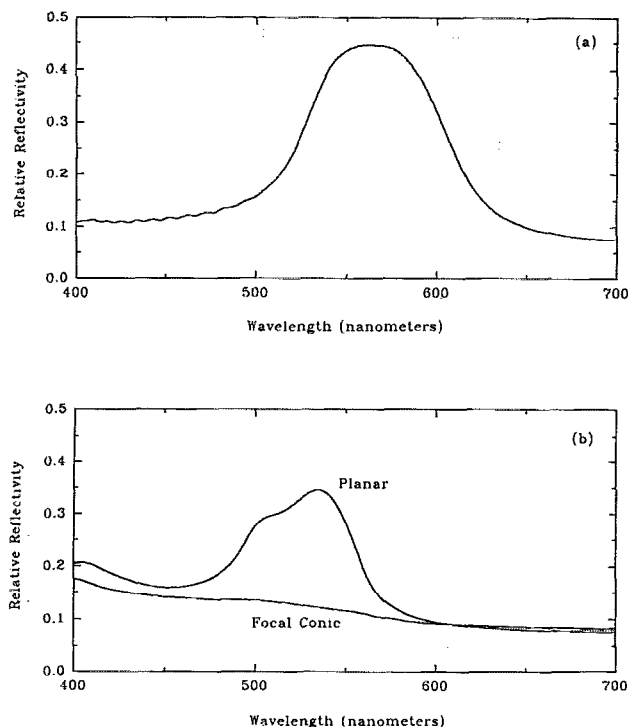
FIG. 2. Relative reflectivity plotted as a function of wavelength for (a) a chiral nematic mixture composed of CE2/CB15/E48 in a 1:1:3 weight ratio, and (b) a CPD shutter composed of the above chiral nematic mixture and the other components listed in Table I, in either the planar or focal conic state.
