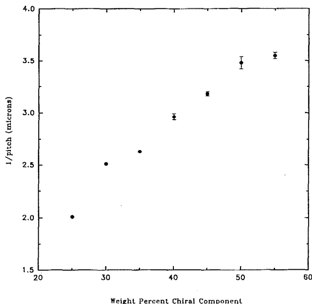
FIG. 1. Pitch length of CPD films in the planar state plotted as a function of the weight percent of the chiral component in the chiral nematic mixture. Each point is an average of three different samples. The standard deviation is indicated by the error bars. The chiral component consists of a 50:50 blend by weight of CE2 and CB15. E48 is the nematic host.
