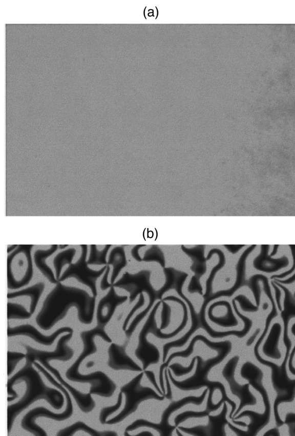
FIG. 3. Polarizing microscopy texture of a homogeneously aligned cell prepared by conventional UV method: (a) before and (b) after thermal annealing at 100 \text{ }^\circ\text{C} for 12 h. The loss of alignment in (b) shows thermal instability of this alignment method.
